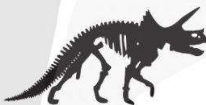
___ skeleton
