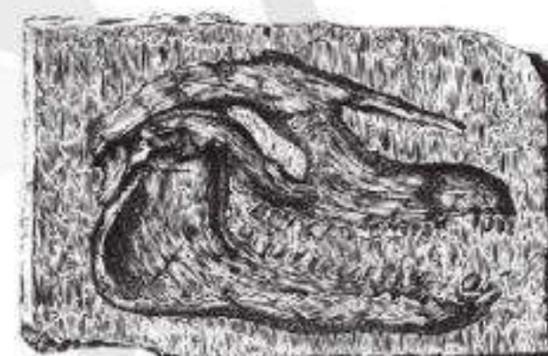
___ fossil
